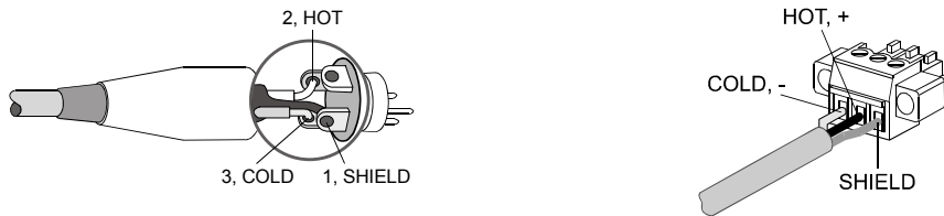
Illustration 2.10: Balanced connection of input
