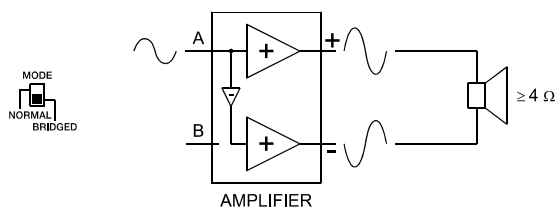
Illustration 2.9: BRIDGED mode
