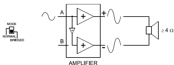
Illustration 2.9 : Mode BRIDGED
