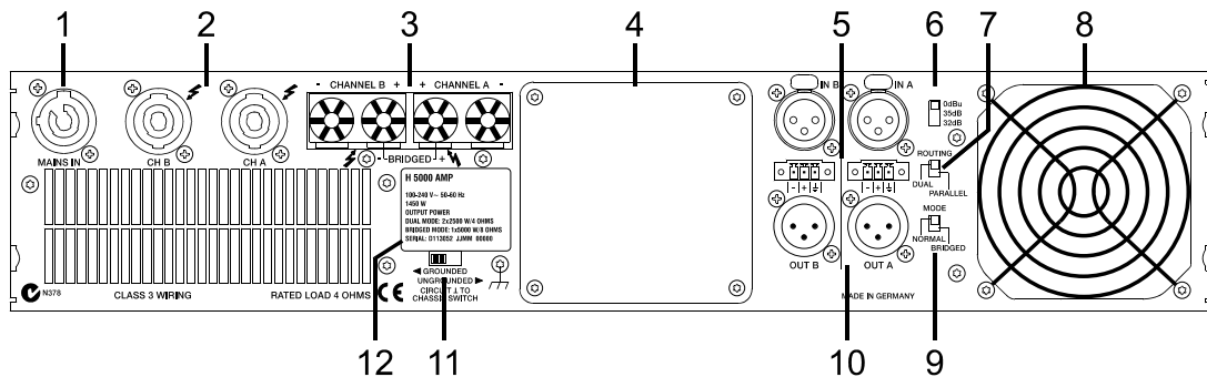
Illustration 2.2: H2500/H5000 rear view
