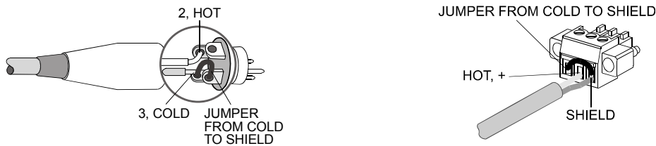
Illustration 2.11: Unbalanced connection of input
