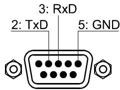
Illustration 4.9: Pin-assignment of RS-232 Interface
