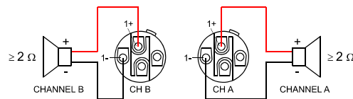
Illustration 2.13: Speaker connection in NORMAL operation mode, using Speakon A and B connectors
