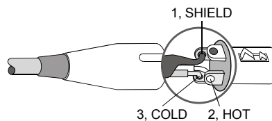
Illustration 2.12: Balanced connection of output (Daisy-Chain)
