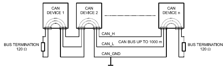
Illustration 4.10: Topologie du bus CAN
