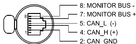
Illustration 4.7: Pin-assignment of CAN jack
