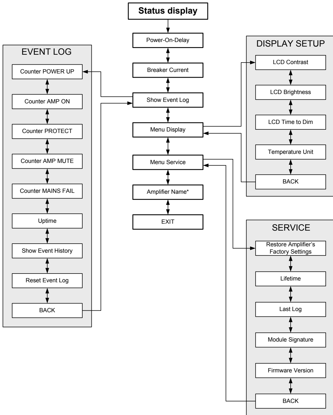
Illustration 3.4: The power amp's menu structure
