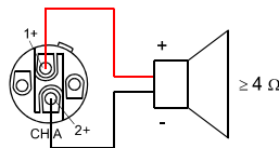
Illustration 2.16: Speaker connection in BRIDGED operation mode, using Speakon A
