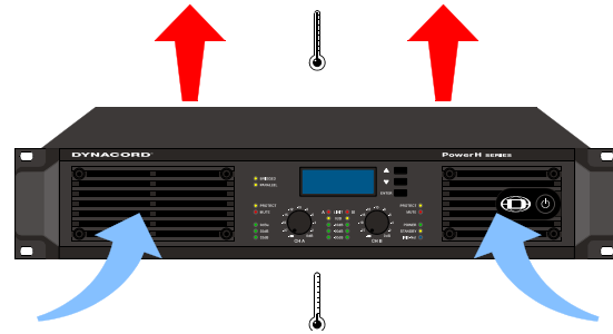
Illustration 2.6: H2500/H5000 Ventilation
