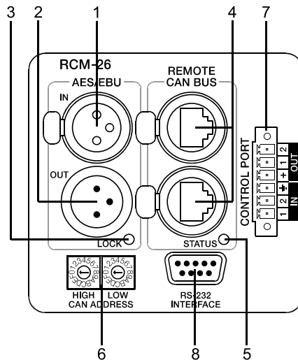
Illustration 4.4: Controls and Connections of the RCM-26
