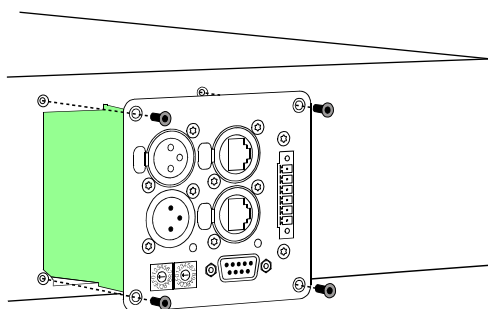
Illustration 4.1: Installation of a RCM-26
