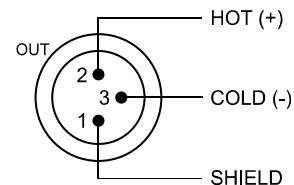
Illustration 4.6: Pin assignment of AES/EBU-OUT
